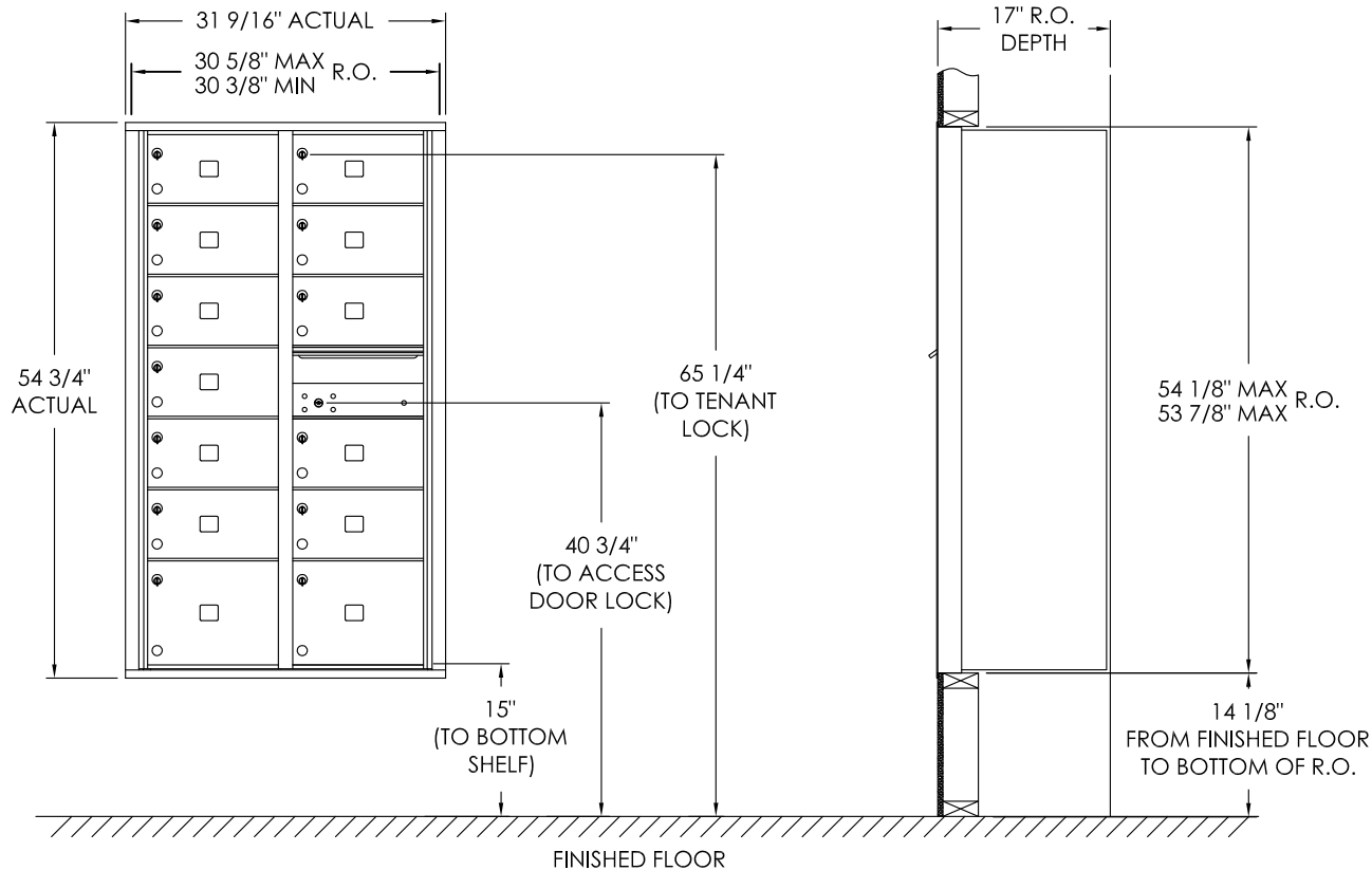
COMPARTMENT CHART
